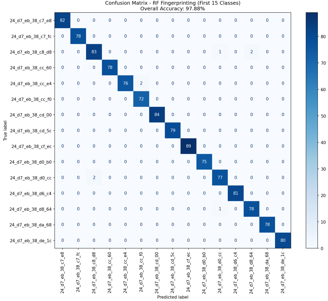
Figure 1.2: Confusion Matrix - RF Fingerprinting (First 15 of 123 Classes)
